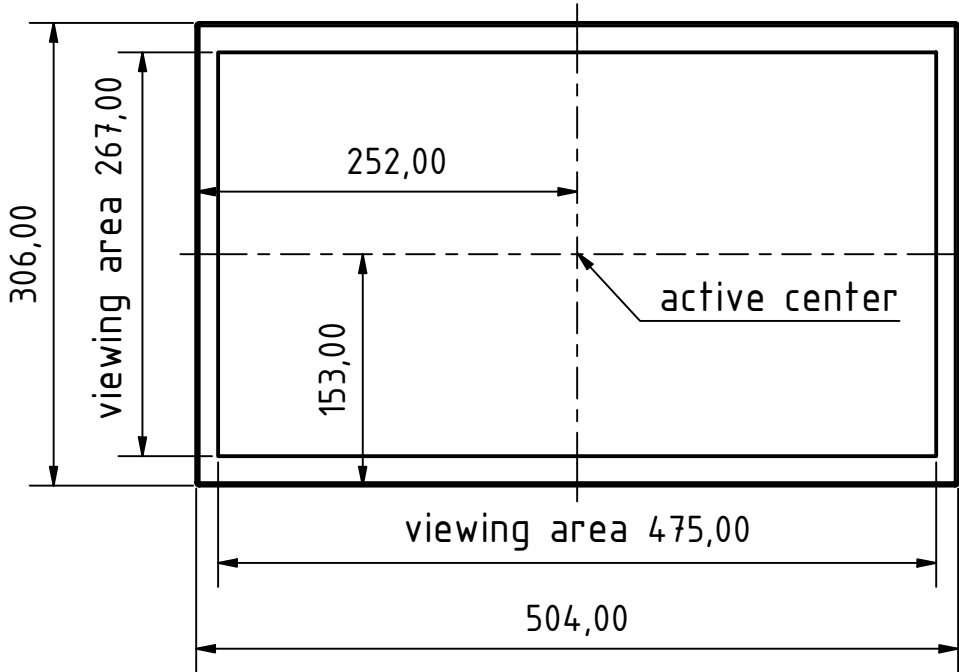
Top View ( 1 : 5 )
