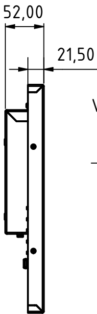
Side View ( 1 : 5 )
